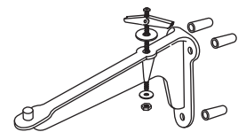
1511 Bolt on pin bracket Code No. 811236 with 50mm Stand off spacer kit Code No. 887711.
