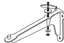
1510/1511 Bolt on pin bracket Code No. 811221/811236.
